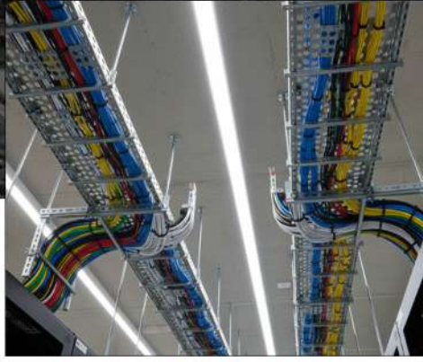
Perforated Cable Tray
