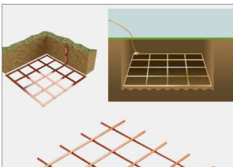
Grid Earthing System
